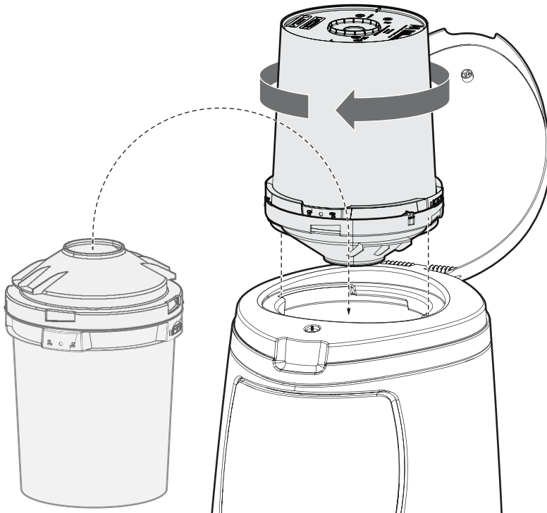
Figure 7. Bucket Funnel Installation
