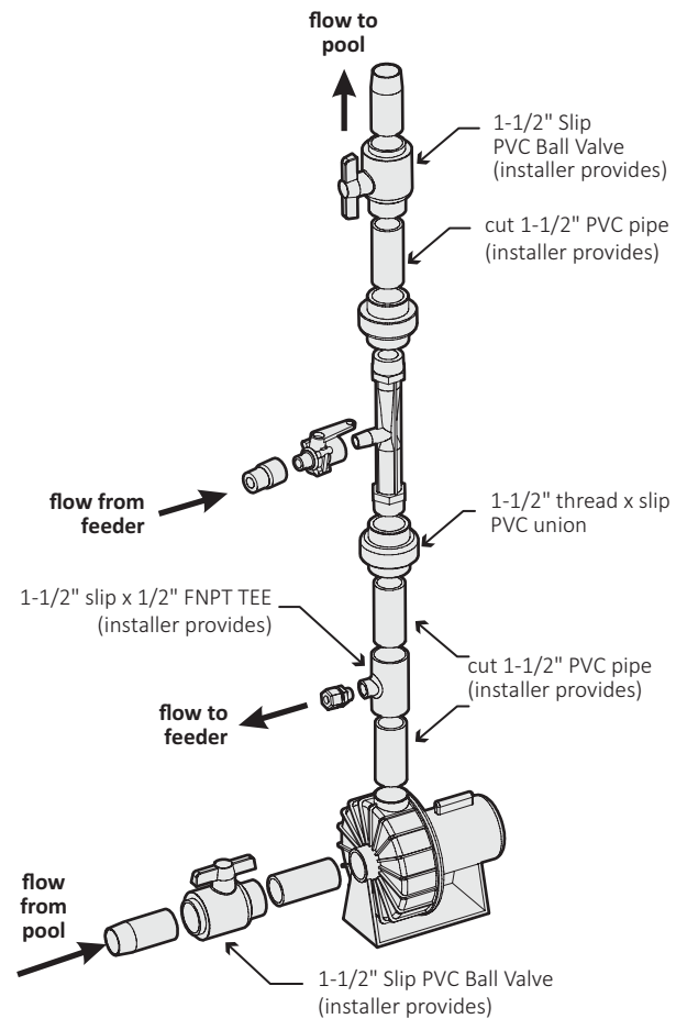
Figure 3. Complete the 1 ½" piping run
