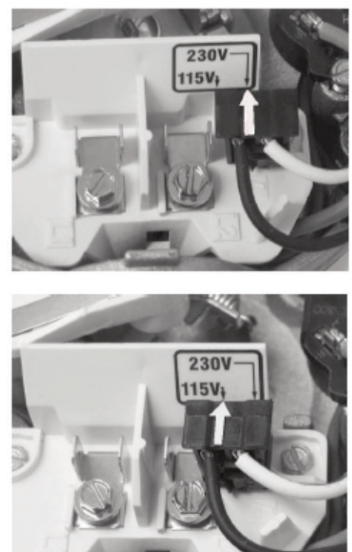
Figure 5. Wire the Booster Pump
